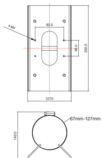
TVB-PM Corner Mount Adaptor for S6 bullet cameras
