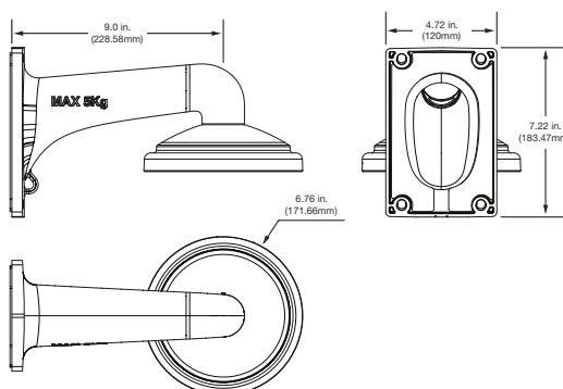
TVP-CCBWM compact cup base PTZ wall mount
