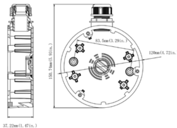
TVW-BB1 S6 wedge back box
