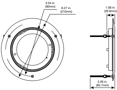
TVD-VFM dome flush mount
