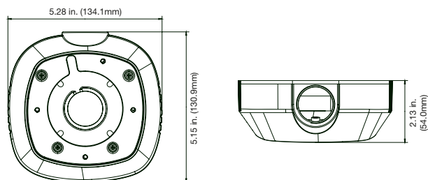
TVW-AWB-1 angled outdoor back box
