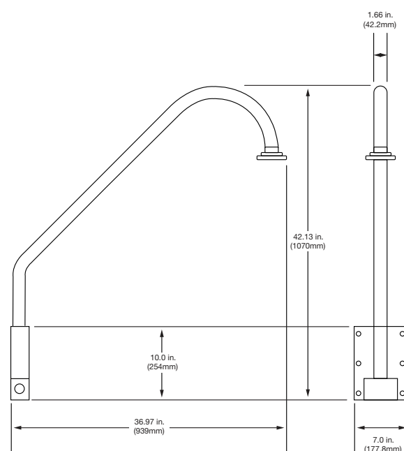
TVP-SAM PTZ swing arm mount
