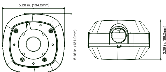
TVW-DVM dual view mount
