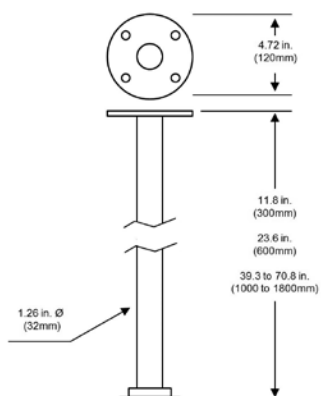
UVP-C30/C60/C180 ceiling mount
